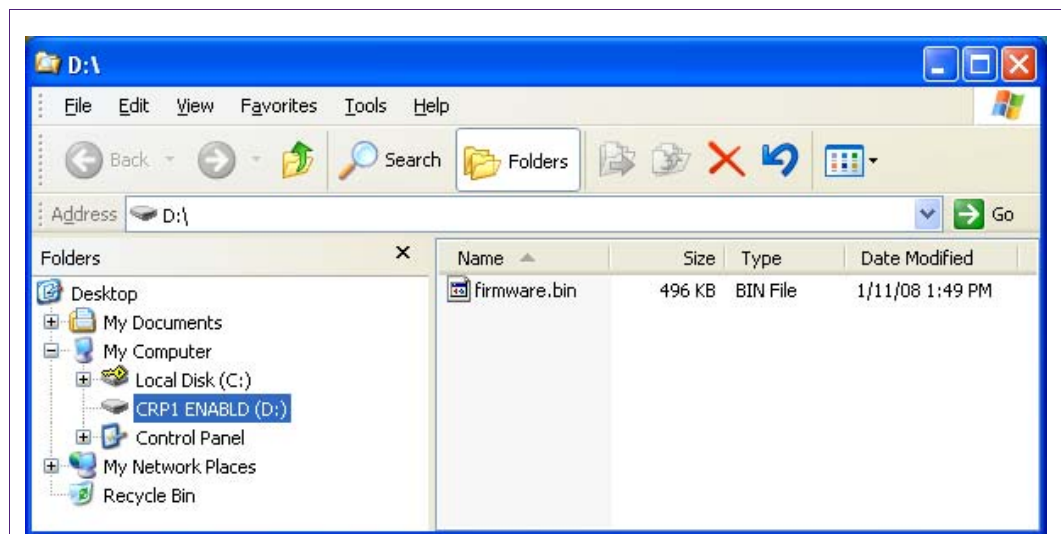
Fig 7. CRP1 screenshot
