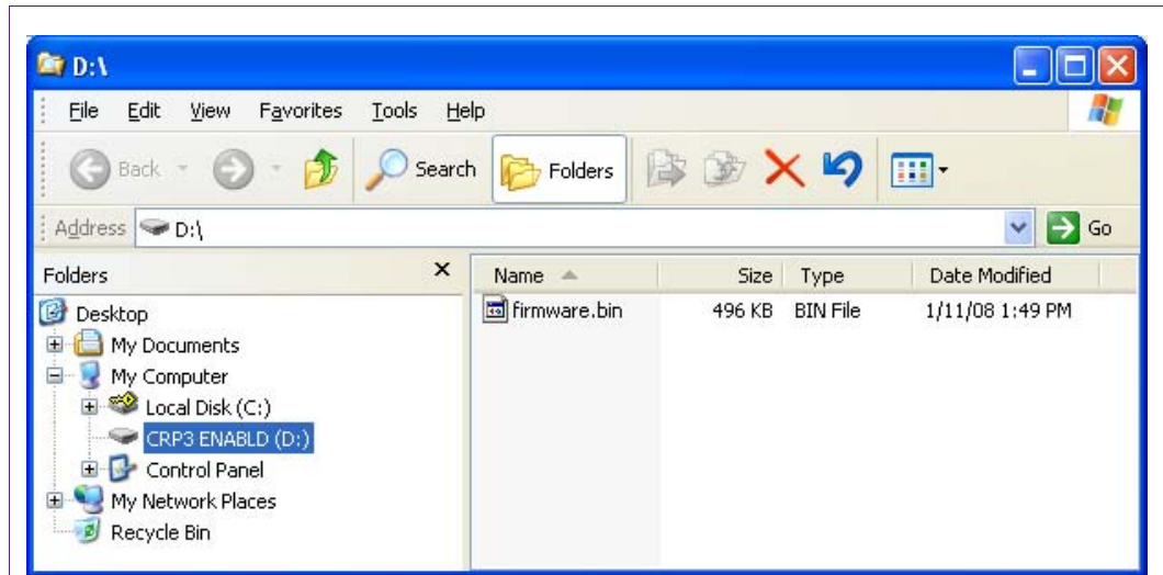
Fig 9. CRP3 screenshot
