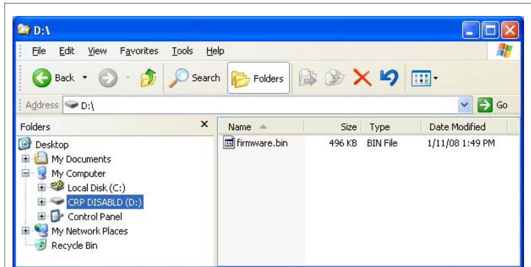
Fig 6. firmware.bin screenshot
