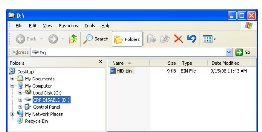
Fig 5. USBHID.bin screenshot
