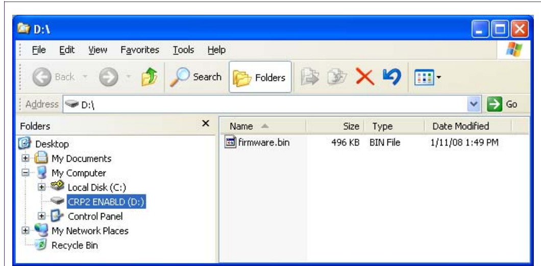
Fig 8. CRP2 screenshot
